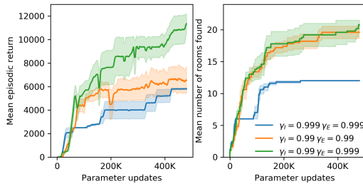
Figure 5: Performance of different discount factors for intrinsic and extrinsic reward streams. A higher discount factor for the extrinsic rewards leads to better performance, while for intrinsic rewards it hurts exploration.
