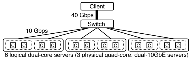
Figure 8: Experimental topology.
