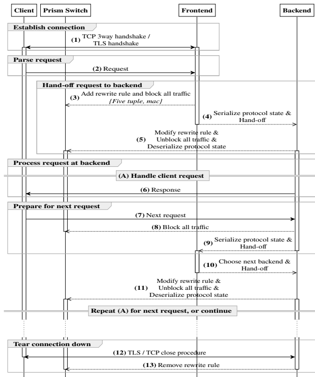
Figure 4: End-to-end Prism operation. Solid arrows indicate TCP packets, dashed ones control messages. Step (8)–(11) indicates our two-phase hand-off protocol described in Section 4.2.
