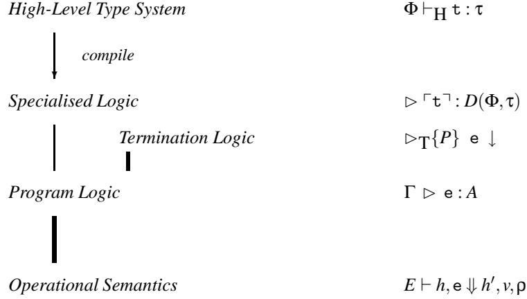
FIGURE 14.1. A family of logics for resource consumption
