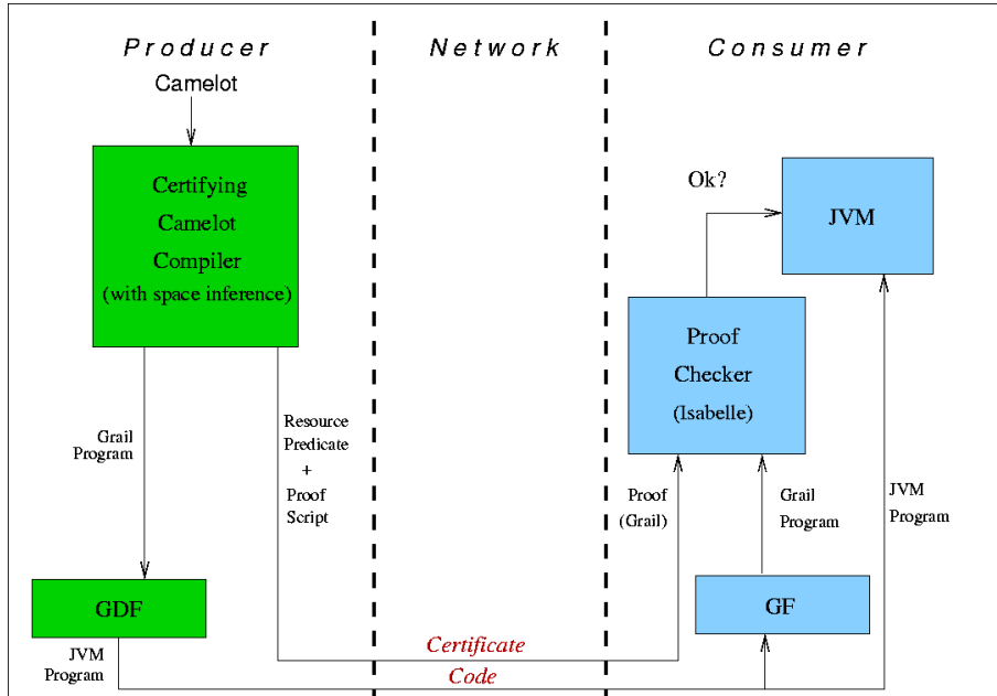
FIGURE 14.5. PCC infrastructure for MRG
