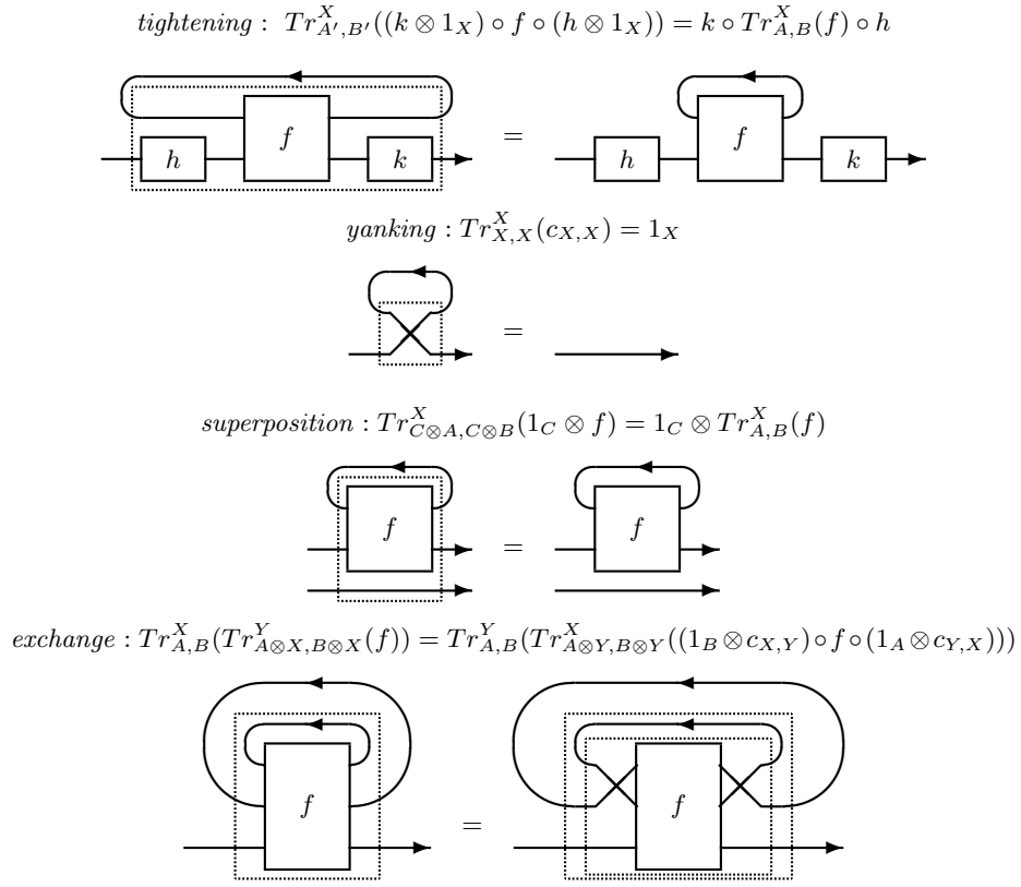
Fig. 1. Axioms for Trace
