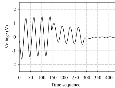
Fig. 9. Recorded signal waveform on a pair of electrodes without OZS timing control.
