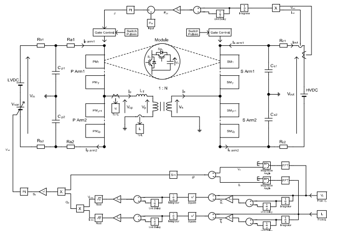
Fig 4: Detailed MMC model and closed loop control
