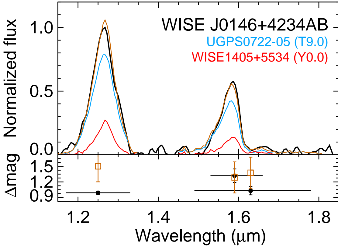
Fig. 3.— Integrated-light spectrum (black) and best matching component templates (colored lines). The bottom subpanel shows the observed J -, H -, and \text{CH}_4\text{s} -band broadband flux ratios used to constrain the decomposition (filled black circles with errors) and the resulting flux ratios computed from the best matching template pair (open brown squares).
