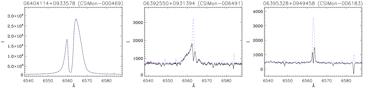
Fig. 1. Original (lilac dashed line) and sky-subtracted (black line) spectra for three cases: good case without a flag from the tool (left panel); intermediate case, with flag from the tool and broad H\alpha line profile (middle panel); a case with flag from the tool and narrow H\alpha line profile (right panel).
