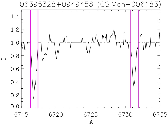
Fig. A.2. The range of the spectrum of one object around the [SII] doublet: our tool allows to select those objects with spurious absorption features, as highlighted by the vertical magenta lines around the absorption lines in this figure.
