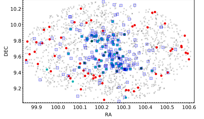
Fig. 5. Spatial distribution of all the targets (gray crosses) here investigated: blue empty squares are the confirmed accretors, green and red dots are the good and bad cases, respectively.
