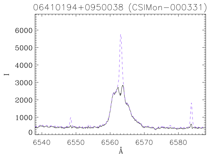
Fig. 4. The range of the spectrum around the H\alpha line including also the [NII] doublet for a non-flagged OH \alpha NA case. The original spectrum is shown in lilac dashed, the sky-subtracted spectrum in black.
