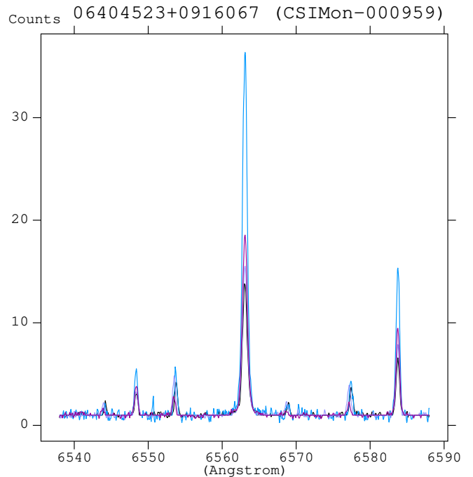
Fig. 7. Variability of the spectrum near the H\alpha emission line of the OH \alpha NA not flagged class II accretor 06404523+0916067 for the original spectra with FWZI greater than pure nebular contribution: different colours correspond to spectra collected in different observations of the same object.
