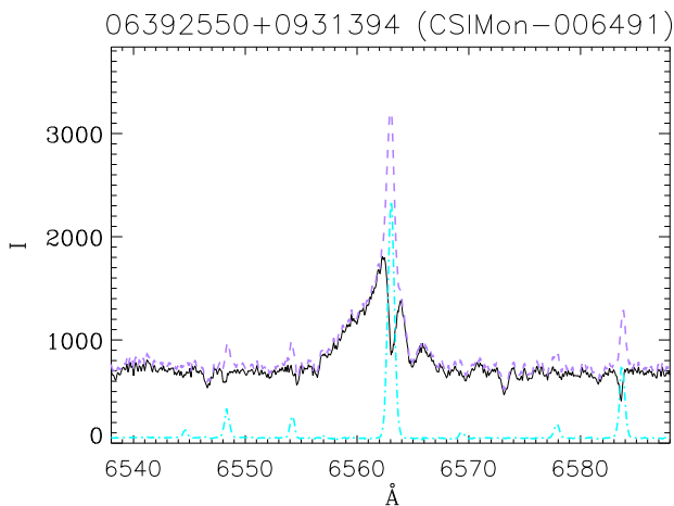
Fig. 2. The range of the spectrum of the object 06392550+0931394 (same object as that shown in Fig. 1, middle panel) around the H\alpha line including also the [NII] doublet. The original spectrum is shown in lilac dashed, the sky-subtracted spectrum in black, and the nebular contribution used for the sky subtraction is in cyan dashed-dotted.
