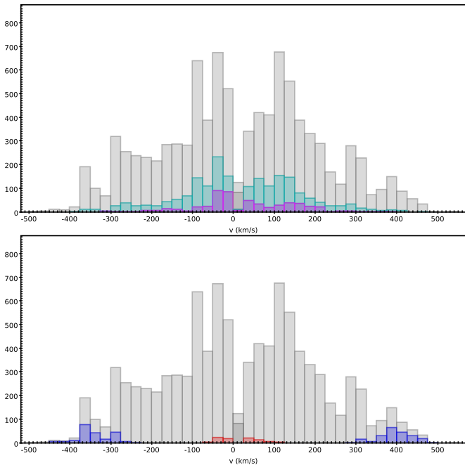
Fig. 6. Histograms as a function of the velocity derived from the wings of the H\alpha line for the spectra with S/N > 10 . Upper panel: the flagged spectra with spurious absorption doublets are highlighted in light blue for [SII] and in magenta for [NII]. Lower panel: good (blue) and bad (red) cases are highlighted.
