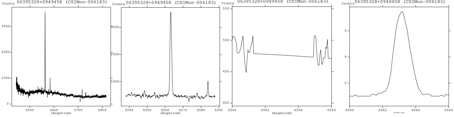
Fig. A.1. The steps to isolate the line of interest: 1) total spectrum (first panel); 2) the zoomed spectrum (second panel); 3) the spectrum with suppression of the line (third panel); 4) the isolated line (fourth panel).
