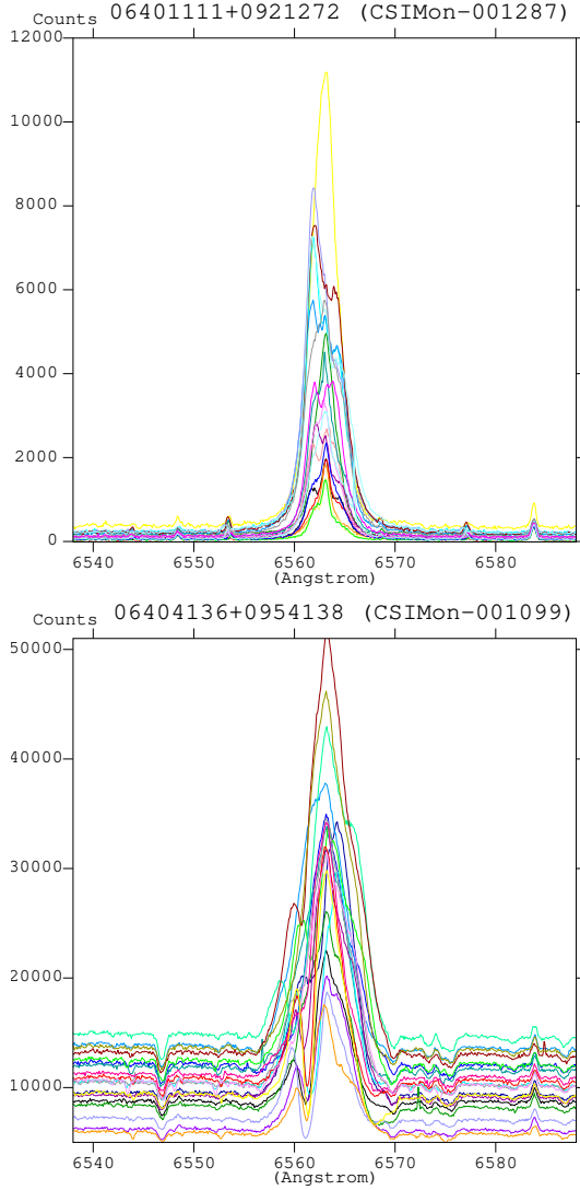
Fig. 8. Variability of the spectrum near the H\alpha emission line of the intermediate accretor 06401111+0921272 (upper panel) and of the class II accretor 06404136+0954138 (lower panel) for all the 20 the original spectra collected for each of these stars. (Note that to avoid confusion, the spectra are not continuum normalized and the continua are therefore different)
