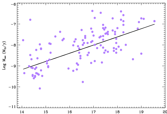
Fig. 9. \log(\dot{M}) derived from the H\alpha_{10\%} following the Natta et al. 2004 as a function of the FWZI for the good cases, the confident accretors, with high S/N ( > 40 ), and H\alpha_{10\%} > 200 km/s, whose spectra are not altered by the nebular contribution and therefore allow us to derive reliable measurements from their peak. The data of the good cases are shown as lilac dots and the best-fit line is superimposed.
