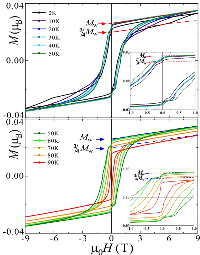
FIG. 3. Magnetization-field hysteresis loops for YRuO_3 with loops between 2 and 50 K and between 50 and 90 K separated for clarity. Insets show low-field data. The saturated weak magnetization M_w and the \frac{3}{4}M_w quantum weak ferromagnetic features are labeled. M_w is linearly extrapolated from the high-field magnetization to H = 0 as shown and the \frac{3}{4}M_w line is drawn parallel to the M_w line with M = \frac{3}{4}M_w at H = 0 .
