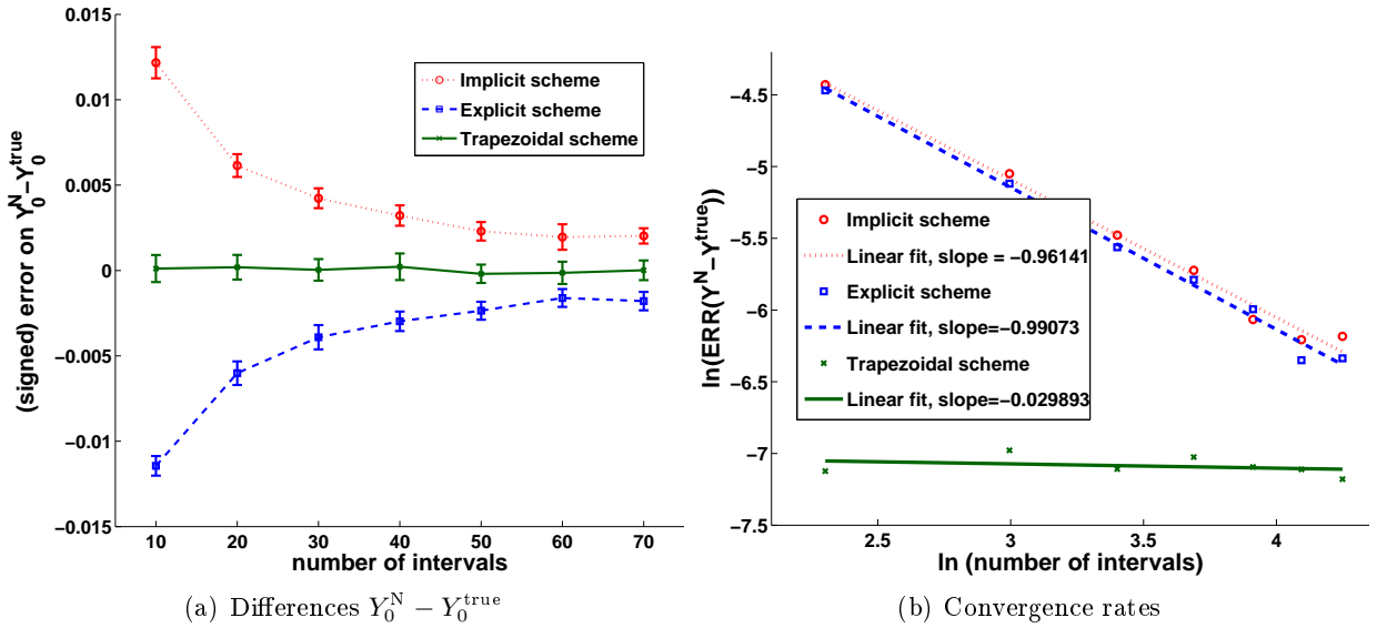
Figure 1: (a) Differences Y_0^N - Y_0^{\text{true}} for each scheme as functions on the number N of time intervals. (b) Convergence rates obtained via linear fits on the log-log plots of ERR(Y^N) . We used N \in \{10, 20, 30, 40, 50, 60, 70\} , Hermite polynomials up to degree K = 7 , M = 2 \times 10^5 and 10 simulations for each point.
