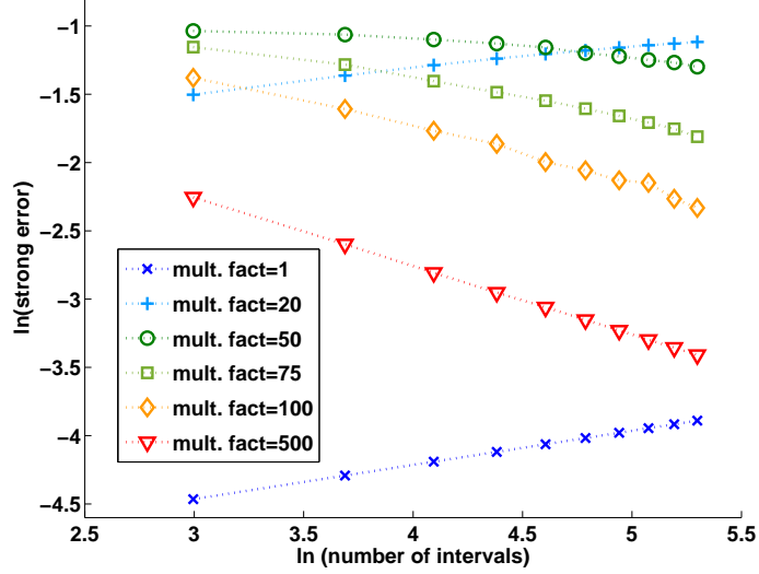
Figure 3: Convergence of the error \mathbb{E}[|T_{L_N}(g(X_N^N)) - T_{L_{2N}}(g(X_{2N}^{2N}))|^2]^{1/2} on the terminal condition, computed for N \in \{20i : i = 1, \dots, 10\} . Plot in log-log scale with different levels of truncation L_N = \alpha L_h , done with M = 10^5 and 10 simulations for each point. The estimated slopes are, for the corresponding multiplicative factors: 0.25, 0.17, -0.12 , -0.29 , -0.41 , -0.50 (reading the legend from top to bottom).
