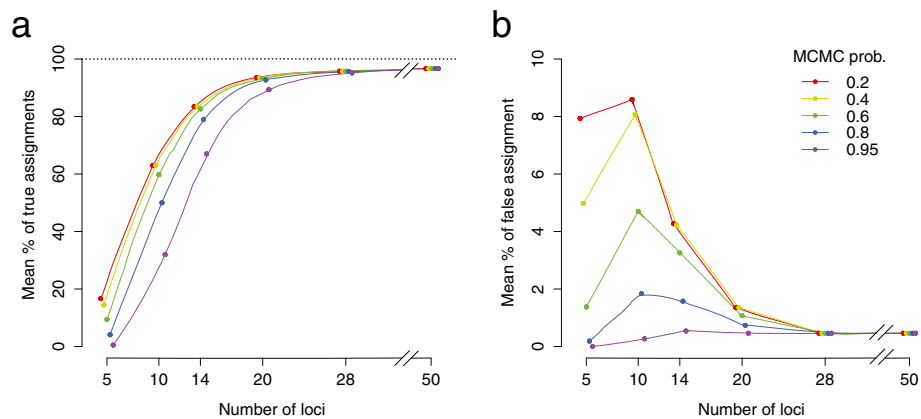
Figure 4 Assignment success as a function of marker number. (a) True assignment per cent. (b) False assignment per cent. Each data point is the mean of simulations of six parent-offspring cohort pairs, in which genotypes at each cohort pair were simulated 100 times using empirical allele frequency distribution. The points are jittered on the x axis to improve visual interpretation.
