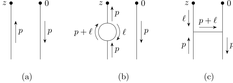
Figure 2.2. Feynman diagrams up to one loop for \langle 0|T[\phi(z)\phi(0)\phi(z_1)\phi(z_2)]|0\rangle .
