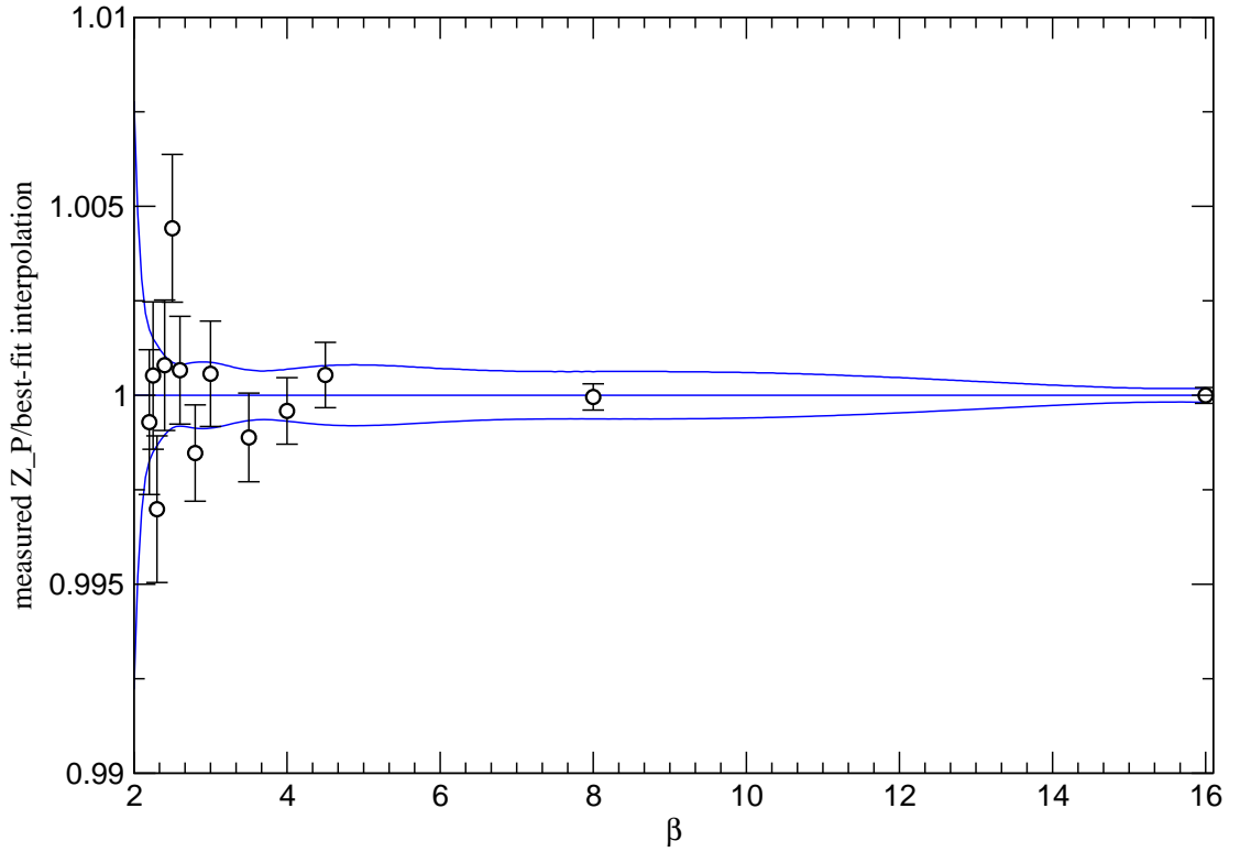
Figure 11: Example of an interpolation function for L = 8 , with a \pm\sigma confidence interval, compared with measured Z_P data points.
