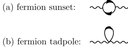
Figure 2: Fermionic contributions to the gluon two-point function.
