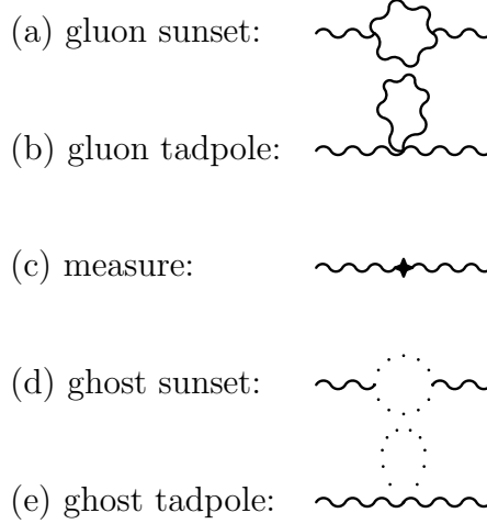
Figure 1: Contributions to the gluon two–point function in the pure gauge theory.
