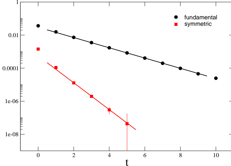
Figure 2: Correlator data for the fundamental (circles) and symmetric (squares) representations, with L = 12 , as a function of the temporal distance t . Solid lines are exponential fits to data with t \geq 3 , leading to markedly different values of m_k .
