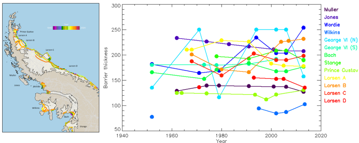
540 Figure 3 Change in Antarctic ice shelf barrier position (left) and thickness (right) over time. Barrier positions are derived from episodic satellite imagery (Cook and Vaughan, 2010), and barrier thicknesses are derived from airborne ice penetrating radar (light grey lines) and satellite radar altimetry (Fretwell et al., 2013).
