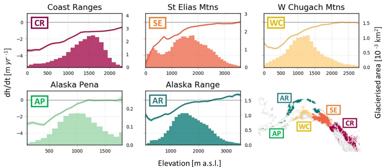
Figure 11: Altitudinal distribution of elevation changes and glacier hypsometry functions in the Gulf of Alaska (GoA) in RGI 6.0 sub-regions between 2010 and 2019. The lines show elevation change rates with uncertainty envelopes plotted against 100 metre elevation bands (left y-axis). The bars display the glacier hypsometry (right y-axis).
