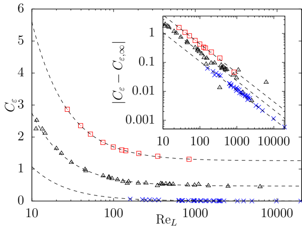
FIG. 5: Main panel: C_\varepsilon against Re_L . Dashed line fit for model Equation (6) for two ( \times ), three ( \Delta ) and four ( \square ) dimensions. Inset: |C_\varepsilon - C_{\varepsilon,\infty}| against Re_L , dashed line corresponds to power law behavior.
