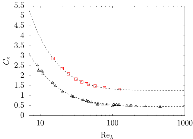
FIG. 6: C_\varepsilon(Re_\lambda) against Re_\lambda . Dashed line fit for model Equation (7) for three ( \Delta ) and four ( \square ) dimensions.
