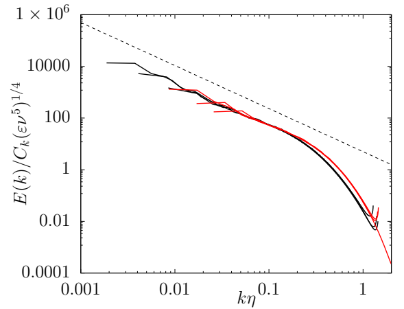
FIG. 1: (Color online) Normalized energy spectrum, E(k) , against k\eta at Re_L = 6207, 2517 and 979 for 3D (black) and Re_L = 838, 347 and 203 for 4D (red). Kolmogorov k^{-5/3} predicted inertial range scaling (long-dashed black).
