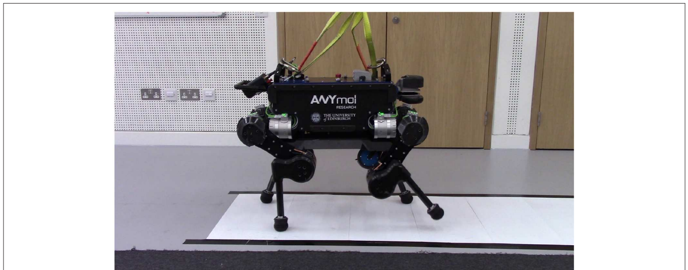
FIGURE 7 | ANYmal walking on slippery synthetic ice. The estimated friction coefficient between ANYmal's feet and the synthetic ice is 0.22. The friction coefficient in our controller needs to be \leq 0.2 in order to avoid slipping on the synthetic ice.
