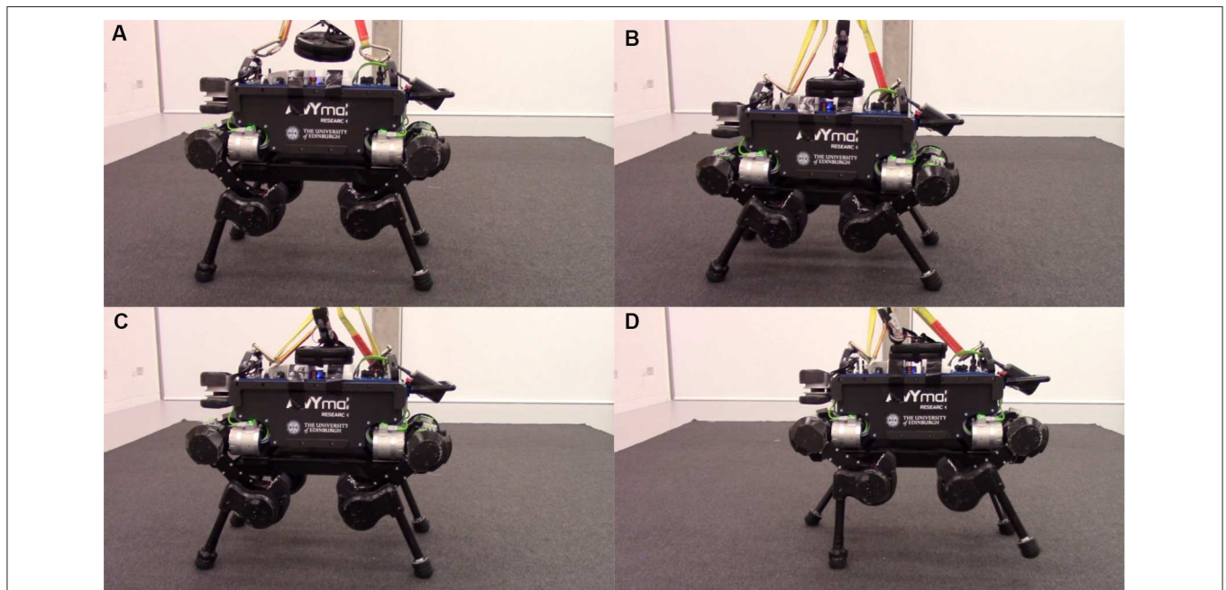
FIGURE 5 | Snapshots of carrying 10 kg weight with model error compensation. (A) Before adding the weight. (B) After adding the weight, the torso went down. (C) The torso went up after enabling model error compensation. (D) Walking with the object with model error compensation.
