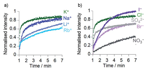
Fig. 4 Ionophoric activity of Cu(II)[ 2 ]Cl 2 (6 \mu\text{M} ) determined through HPTS assays in the presence of different salts (all 100 mM): (a) KCl (●), NaCl (●), LiCl (●), RbCl (●); (b) KCl (●), KI (●), K 2 SO 4 (●), KBr (●), KNO 3 (●). Compounds added at 0 min, base pulse at 1 min, TX-100 addition at 7 min allows data normalisation.
