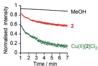
Fig. 5 Lucigenin assays of Cl - transport by MeOH (●), 2 (10 \mu\text{M} , ●) and Cu(II)[ 2 ]Cl 2 (10 \mu\text{M} , ●) with interior NaNO 3 (200 mM) and exterior NaCl (2 M). Compounds added at 0 min, NaCl added at 1 min, TX-100 addition at 7 min allows data normalization.
