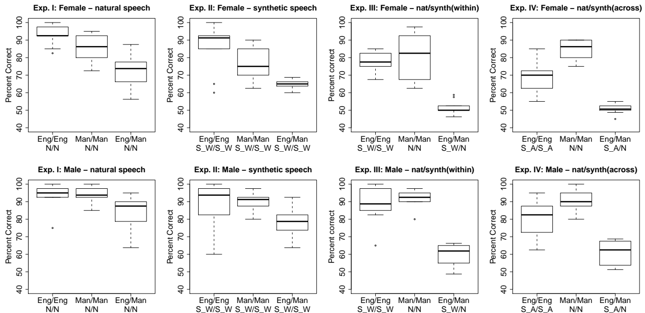
Figure 2: Percent correct discrimination per language pair for male and female test conditions for the four different listening tests. N =Natural speech, S =Synthetic speech, _W =Within-language adaptation, _A =Across-language adaptation.
