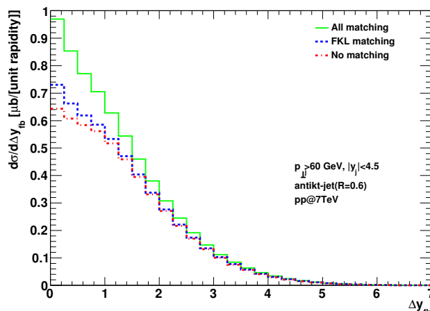
Figure 4. This plot shows the impact of matching in jet production, as a function of rapidity span. The initial HEJ approximation is shown (red, dot-dashed) together with matching to FKL configurations (blue, dashed) and matching to both FKL and non-FKL configurations (green, solid).
