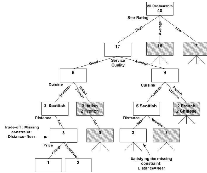
Figure 7: Option tree structure (Option Tree A) corresponding to the User Model A of Table 3. Pruned nodes are shown as shaded.
