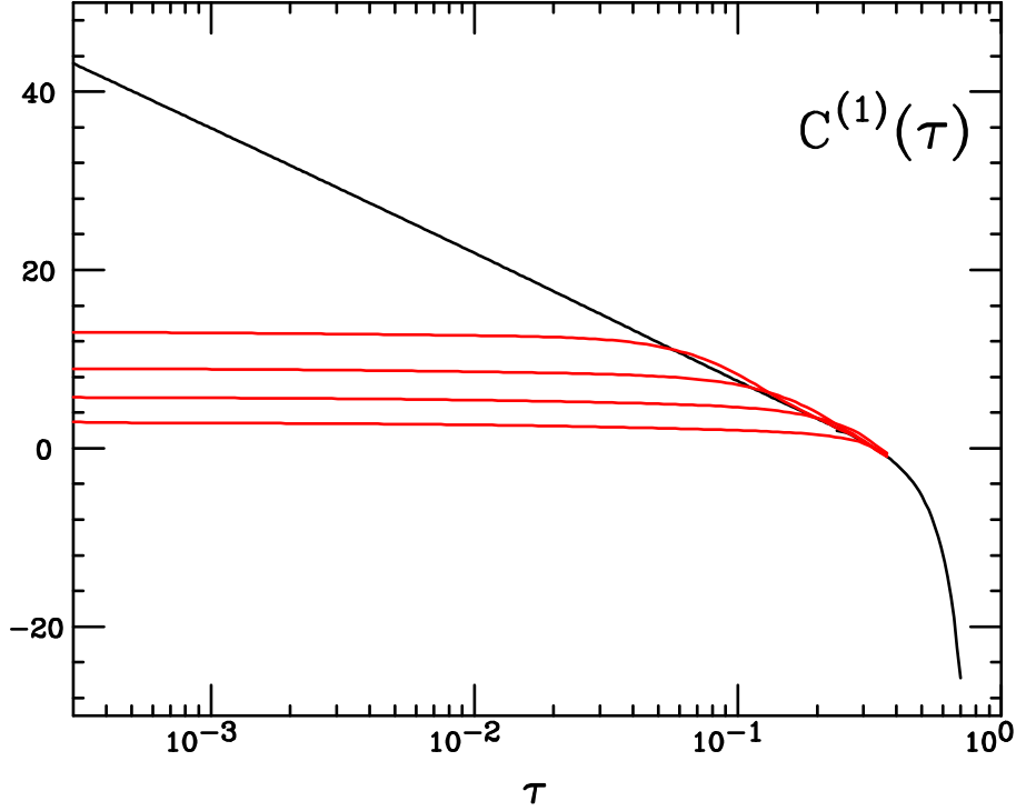
Figure 1: The hard coefficient C^{(1)}(\tau, y_t) eq. (9) (parton-level coefficient function normalized to the Born result) plotted as a function of \tau . The curves from top to bottom on the left correspond to m_t = \infty (black), and to m_t = 170.9 GeV (red), with m_H = 130, 180, 230, 280 GeV.
