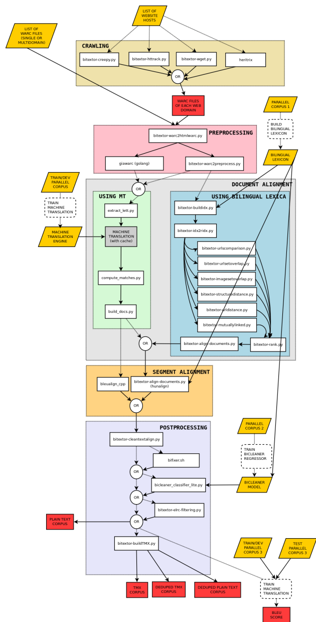
Figure 1: Workflow diagram of Bitextor
