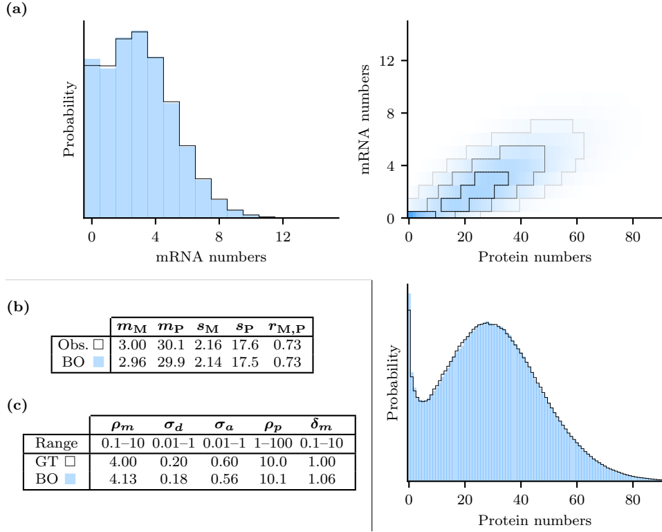
Figure 4: Results for the three-stage gene expression model in Eq. (24). (a): Steady steady state distribution over mRNA and protein numbers for the observed data (contours) and the parameters estimated using Bayesian optimization (shaded). (b): Means ( m ) and standard deviations ( s ) of mRNA and protein numbers as well as their Pearson correlation coefficient ( r ). Both the shape and the moments of the observed distribution are matched by our method. (c): Ground truth and estimated parameters for the observed data and the chosen search ranges. The results were obtained after 362 rounds starting with 300 initial samples, where the GP kernel was refit every 75 rounds during optimization.
