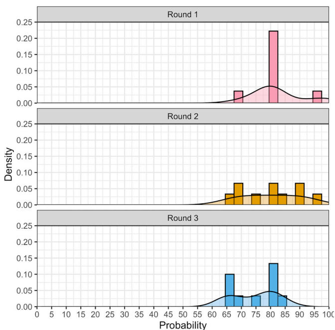
Figure 1 Histogram with density plot demonstrating the voting frequencies from each round.
