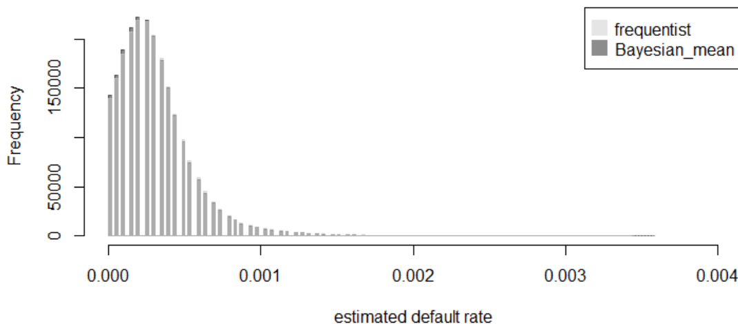
Fig. 3. Histograms of the simulated default rate distributions using frequentist and Bayesian coefficient mean estimates
