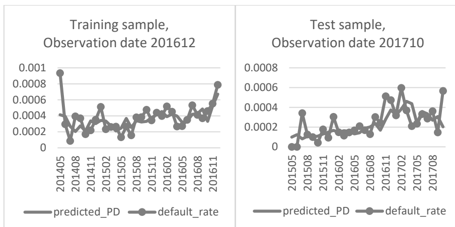
Fig. 2. Predicted and observed DR in the training and test samples using a Bayesian approach
