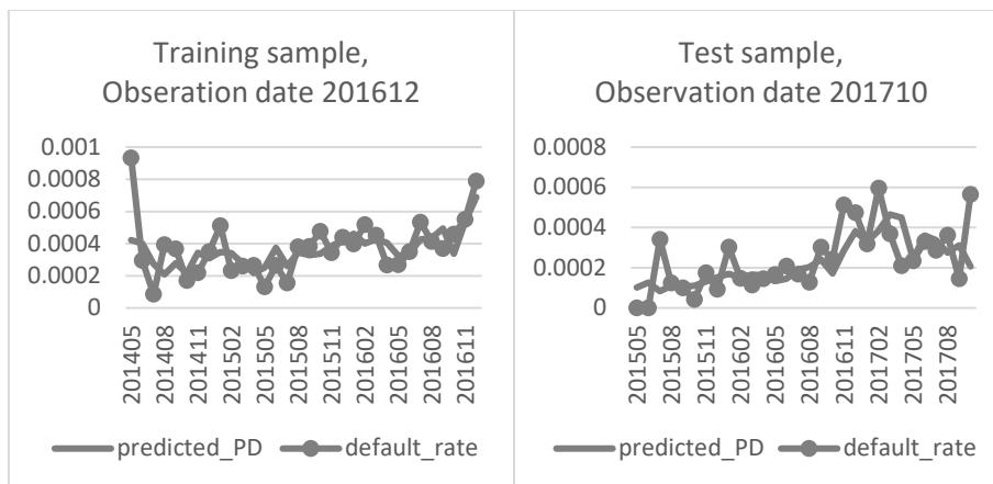
Fig. 1. Predicted and observed DR in the training and test samples using a frequentist approach
