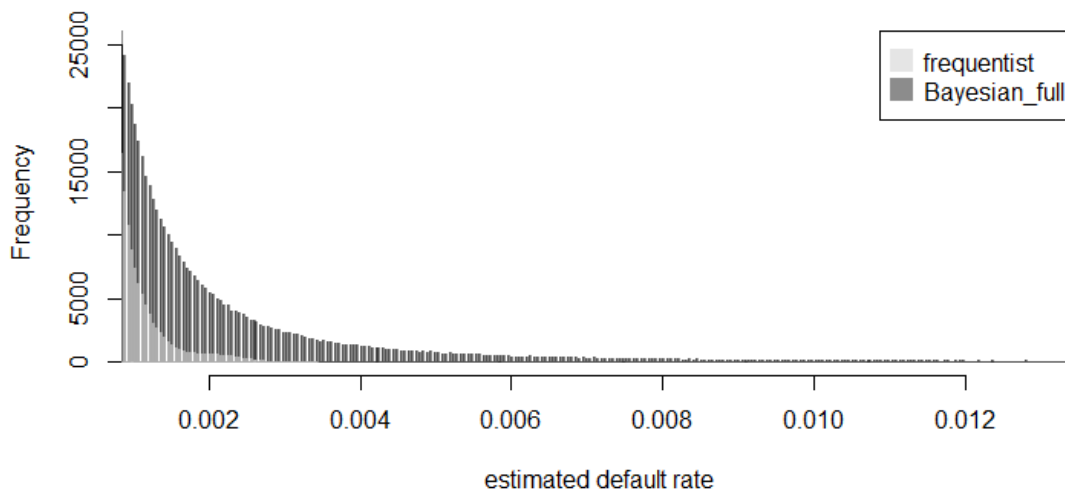
Fig. 5. Tails of the simulated default rate distributions using frequentist coefficient mean estimates and the Bayesian coefficient posterior distribution
