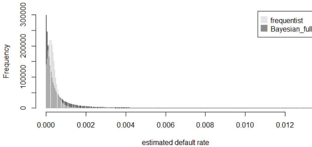
Fig. 4. Histograms of simulated default rate distributions using frequentist coefficient mean estimates and the Bayesian coefficient posterior distribution
