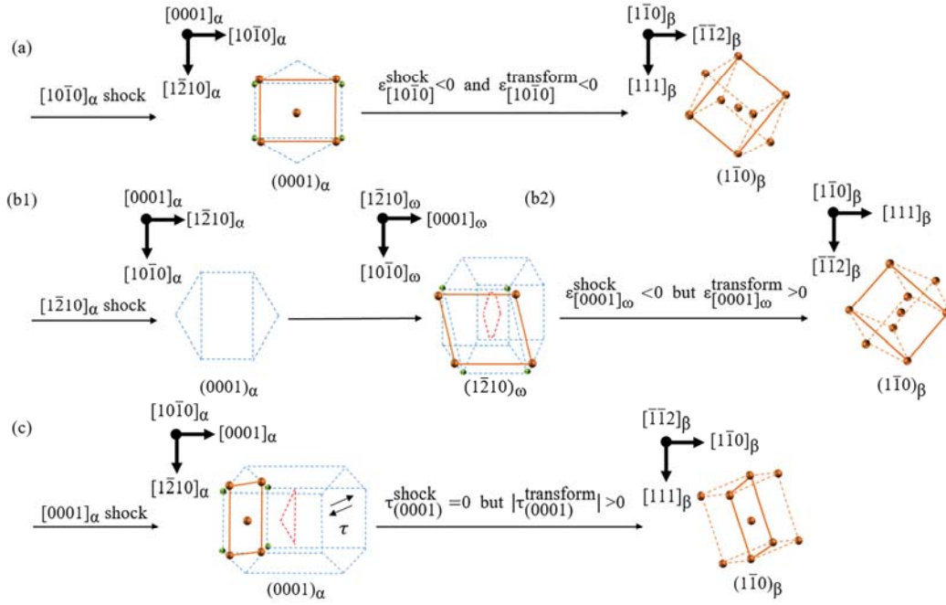
FIG. 12. Schematic illustration of the competition between lattice shape change of phase transformation and uniaxial compression strain of shock loading. (a) The hcp→bcc phase transition requires the hcp-Zr crystal to contract along the [10\bar{1}0] direction, in line with the uniaxial compressive strain applied by shock loading. (b) The strong shock loading along [1\bar{2}10]_\alpha direction leads to a successively hcp → \omega → bcc phase transition. The [1\bar{2}10]_\alpha compressive strain of shock is a barrier for the formation of bcc phase as the phase transition requires a tensile strain along this direction. (c) The c -axial compressive strain of shock can hardly provide any in-plane shear strain that is required for the hcp→bcc phase transition.
