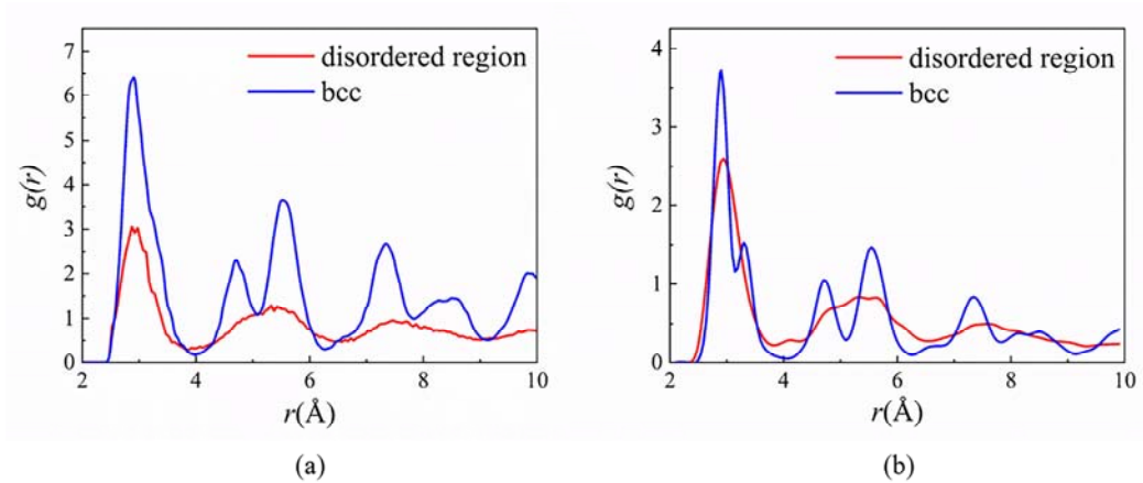
FIG. 5. Comparison of the radial distribution functions (RDFs) of disordered regions and crystallized bcc grains for (a) [0001]_{\alpha} shocked Zr single crystals and (b) [\bar{1}210]_{\alpha} shocked Zr single crystals. It indicates that the disordered regions in both cases have a different structural feature from the bcc phase.
