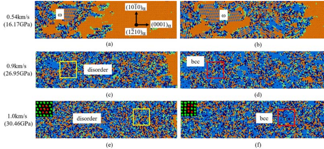
FIG. 4. Snapshots of the phase transformation processes in [0001]_{\alpha} shocked Zr single crystals with different piston velocities. (a) and (b) The nucleation and growth of \omega phase under 0.54 km/s shock compression, intermediated by the formation of metastable bcc. (c) and (d) The formation of bcc phase from the hcp-Zr matrix, accompanied by a few volume fraction of amorphous intermediate. (e) and (f) Under 1.0 km/s shock loading, the hcp-Zr lattices first collapse into obvious disordered region, where new bcc grains forms within the disordered region subsequently. The inset shows the neighborhood information of the atoms before and after the transformation. The color coding are the same with Fig. 2, and the boxes locate the regions for the calculation of local radial distribution functions.
