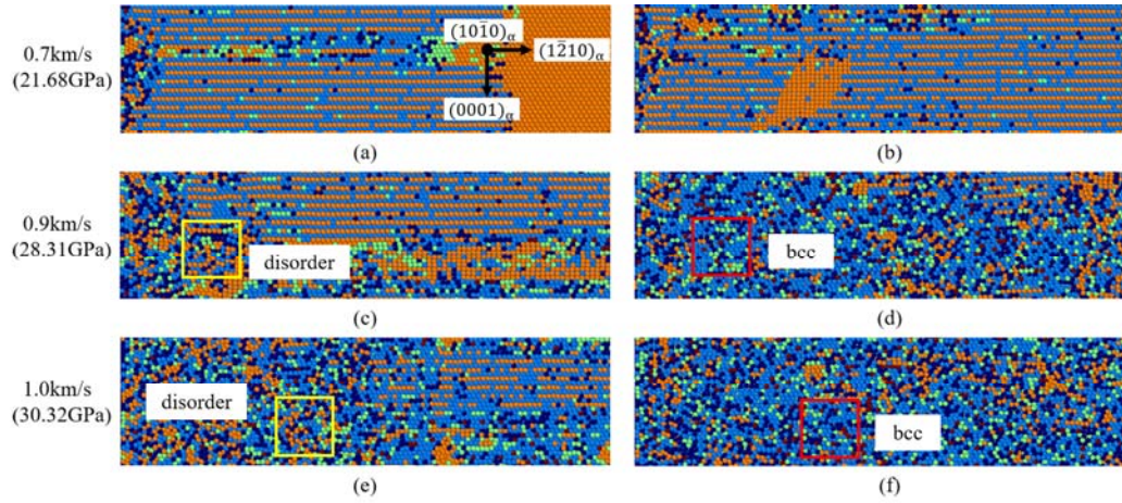
FIG. 6. Snapshots of the phase transformation processes in [\bar{1}\bar{2}10]_{\alpha} shocked Zr single crystals with different piston velocities. (a) and (b) The formation of \omega phase in 0.7 km/s shocked Zr single crystal. (c) to (f) For shock velocity above 0.9 km/s, the \alpha (hcp) \rightarrow \omega phase transformation is followed by the formation of disordered regions, and then new bcc grains forms at the expense of the disordered region. The color coding are the same with Fig. 2, and the boxes locate the regions for the calculation of local radial distribution functions.
