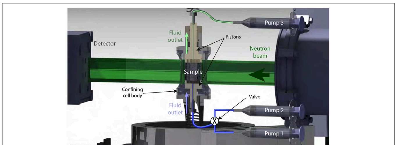
FIGURE 1 | Experimental set-up. A core holder pressurized with nitrogen gas is placed on the rotary stage of the neutron beamline. The sample in the autoclaveA is filled from its bottom side by using one of the two injection pumps. The fluid is recovered by the third pump connected to the top of the sample.
