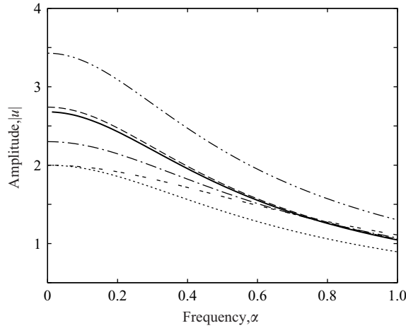
FIGURE 4. Wave-amplitude variation with non-dimensional body-force frequency, \alpha ; Kn = 0.5 . BGK solution (—); Navier–Stokes ( \cdots ); Burnett (---); super-Burnett ( -\cdot-\cdot- ); Grad’s 13-moment ( -\cdot-\cdot- ); regularized 13-moment (---).
