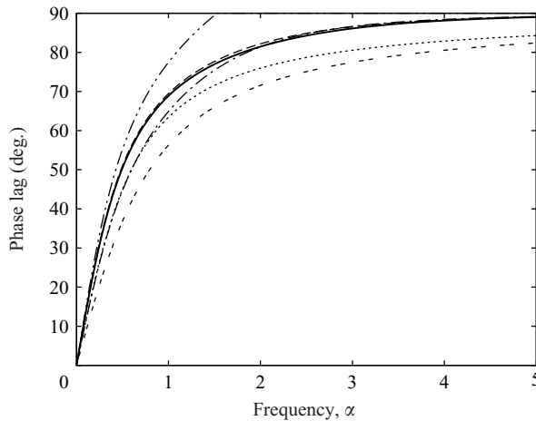
FIGURE 5. Velocity-phase-lag variation with non-dimensional body-force frequency, \alpha ; Kn = 0.5 . BGK solution (—); Navier–Stokes ( \cdots ); Burnett (---); super-Burnett ( -\cdot-\cdot- ); Grad’s 13-moment ( -\cdot-\cdot- ); regularized 13-moment (---).
