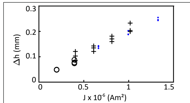
FIG. 3. The change in height ( \Delta h ) between 0 and 0.5 T applied field ( B ) of drops with different total magnetic moments ( J ). The change in height increases with total magnetic moment ( J=\chi VB\mu_0^{-1} ) of a drop with volume V and magnetic susceptibility \chi . The three different markers represent the three salt solutions: 35.6% ppw MnCl 2 (crosses), 17.8% ppw MnCl 2 (circles), and 51.4% ppw GdCl 3 (dots) with \chi = 2.55 \times 10^{-5} , \chi = 1.24 \times 10^{-5} , and \chi = 4.17 \times 10^{-5} respectively.
