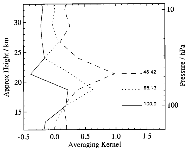
Figure 5. Averaging kernels for 68 hPa and the two levels on either side. The 100 hPa and 46 hPa kernels have been offset by -0.2 and +0.2 , respectively, to make the figure clearer.
