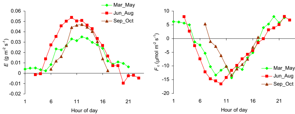
Fig. 4. Daily ensemble means of the elite data set of CO_2 flux ( F_c ) and evaporation rate ( E ) for spring, summer and autumn. The ensemble means were obtained by binning the hourly values for each of the variables for each hour of the days in the monthly periods indicated. The number of values represented by each point varies between 6 and 24. There were fewest observations overnight and fewer at the start and end of each day than in the middle of the day.
