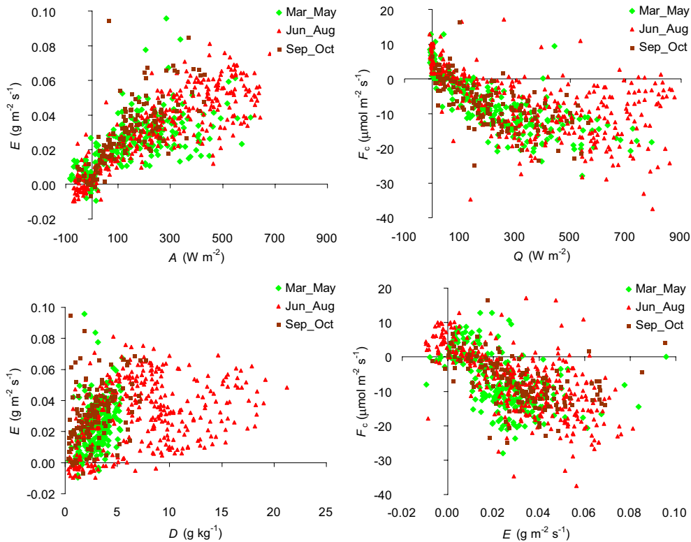
Fig. 5. Scatter plots of the CO_2 flux ( F_c ) in relation to the solar radiation ( Q ) and the evaporation rate ( E ) (right side); and between the evaporation rate ( E ) and the available energy ( A ) and the specific humidity deficit ( D ) (left side). The source dataset is identical to that used in Fig. 4, and is similarly separated into spring, summer and autumn.
