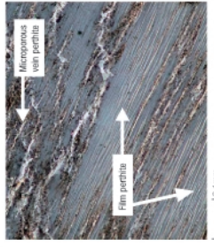
Fig. 2.3 Strain-controlled film perthite, cross-cut by areas of twillite replacement vein perthite. Shear granite, Orick, XP.
