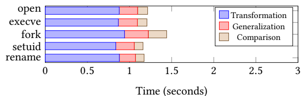
Figure 7. Timing results: CamFlow+ProvJsn
