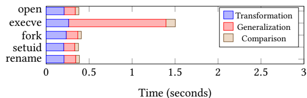
Figure 5. Timing results: SPADE+Graphviz
