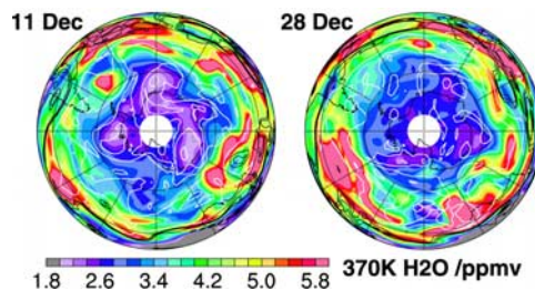
Figure 7. Maps of 370 K MLS \text{H}_2\text{O} ; layout is as in Figure 3. Tropospheric air is equatorward of black PV contours.
