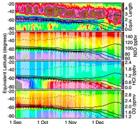
Figure 4. As in Figure 2, but at 520 K (~20 km), and showing MLS N 2 O, HCl, and O 3 .
