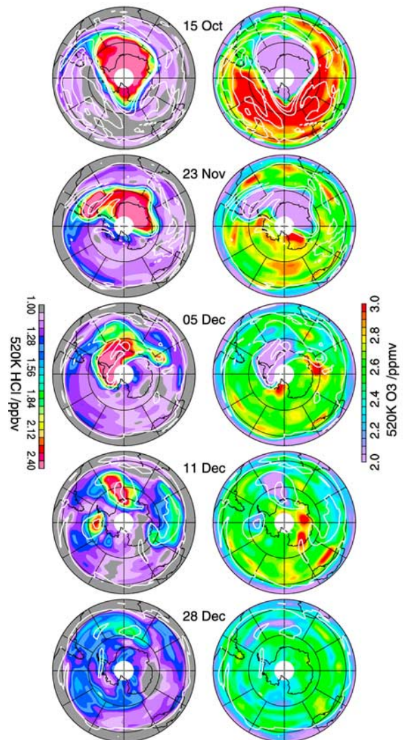
Figure 5. Maps of 520 K MLS HCl and O 3 showing the lower stratospheric vortex breakup. Layout is as in Figure 3.
