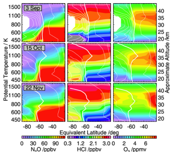
Figure 1. Equivalent Latitude (EqL)/potential temperature cross-sections of MLS \text{N}_2\text{O} , HCl, and \text{O}_3 during the 2004 SH vortex breakup. Overlaid contours are scaled potential vorticity (sPV [Manney et al. , 1994]).
