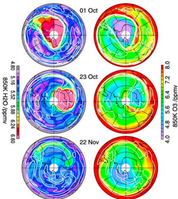
Figure 3. Maps of 850 K MLS H 2 O and O 3 during the vortex breakup. Overlaid contours are sPV. Domain is 0 to 90°S with 0° longitude at the top and 90°E to the right; fine lines show 30 and 60°S latitudes.
