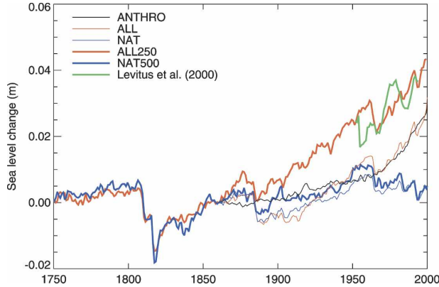
FIG. 6. Annual time series of global-mean sea level change due to thermal expansion from HadCM3 experiments and estimated from the dataset of Levitus et al. (2000) for recent decades. The simulated time series have been shifted vertically so that they all have zero at 1860.
