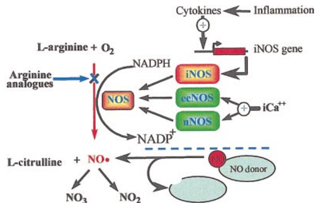
Figure 2. The L-arginine-nitric oxide pathway. NO is synthesized from L-arginine and molecular oxygen by the NOS group of enzymes. In inflammation, cytokines such as IL-1 and TNF are upregulated. The cytokines induce expression of the inducible NOS (iNOS) gene, leading to synthesis of the iNOS enzyme, which produces nitric oxide (NO) from L-arginine. NO can also be produced by pharmacological NO donors such as SNAP. NO is a very reactive molecule and rapidly reacts with oxygen to form nitrite and nitrate.
