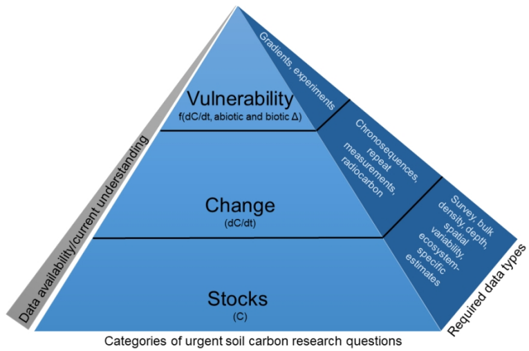
Categories of urgent soil carbon research questions
