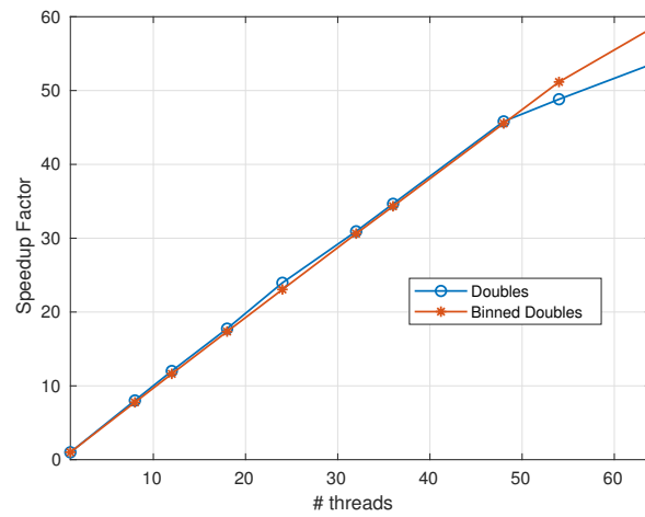
Fig. 4. Comparison of speedup factor of Conjugate Gradient solver for built-in doubles and binned doubles with K = 3 on Fulhame.
