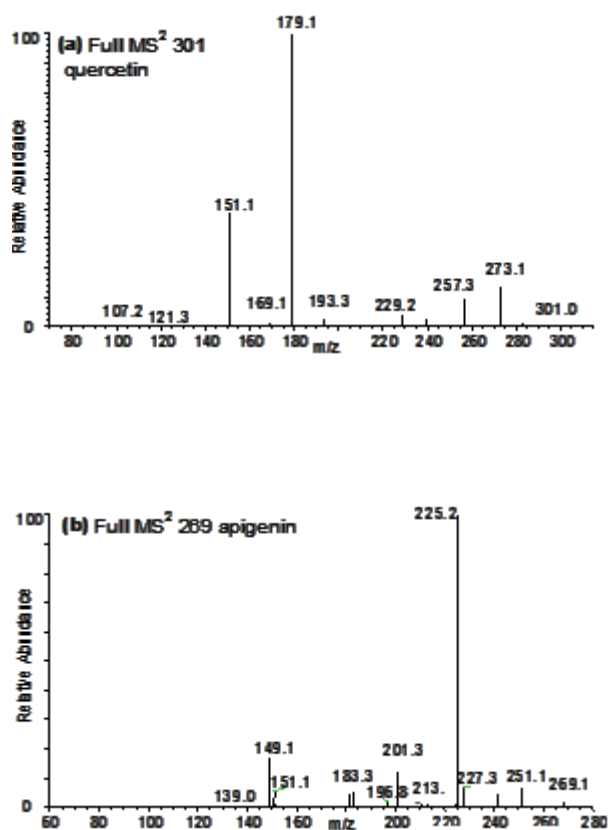
Figure 9. LC-ESIMS analysis of green wool warp thread from the Glencoe tartan fabric. (a) MS 2 m/z = 301 (b) MS 2 m/z = 269.
