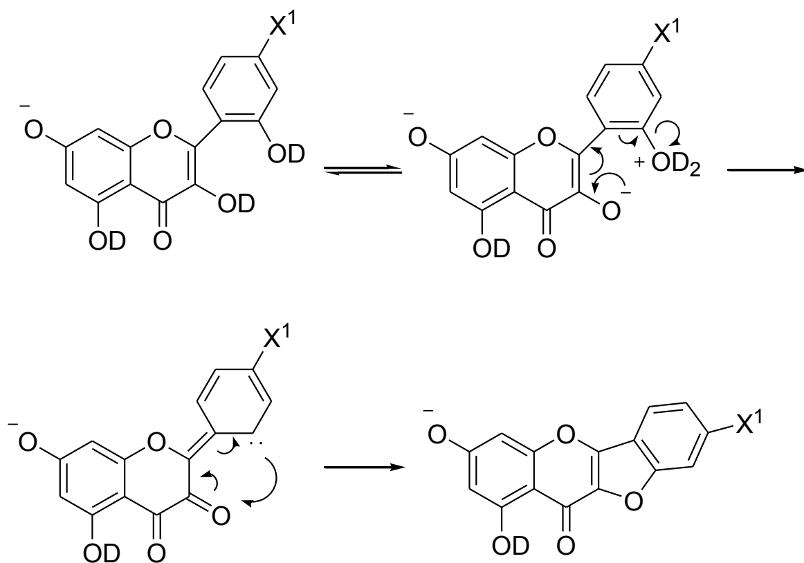
Figure 2. Specific (M-H 2 O) - breakdown mechanism for 2'-hydroxyflavonols.
