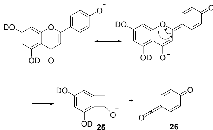
Figure 7. Formation of the m/z 149 fragment ion of 4'-hydroxyflavones.
