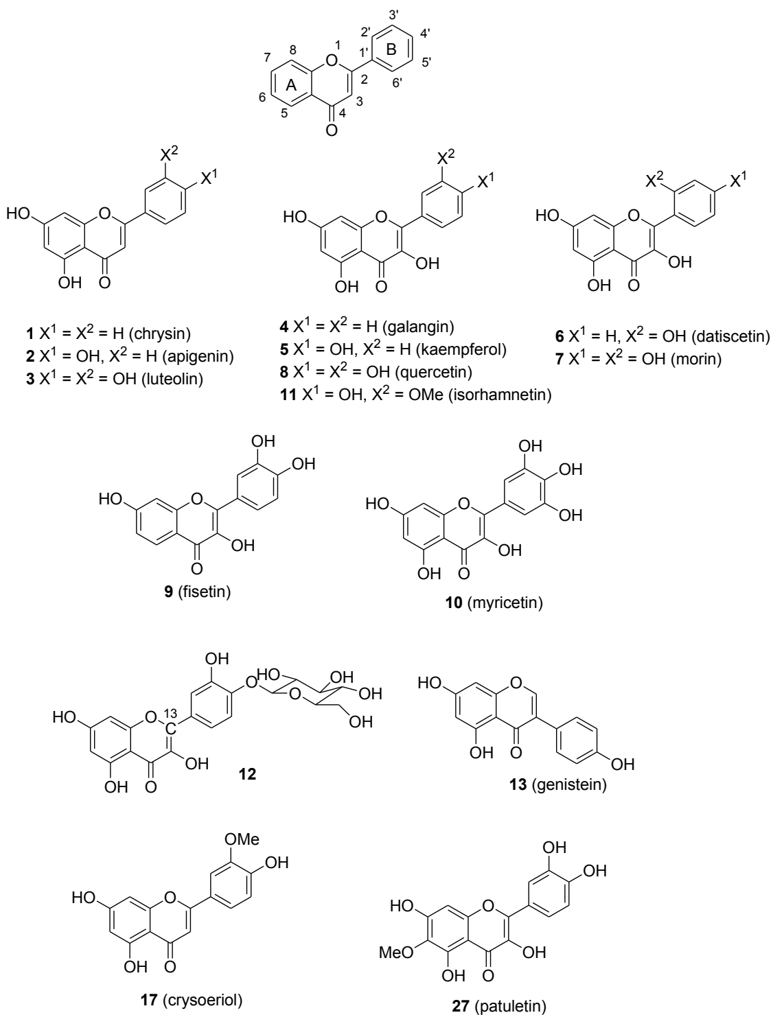
Figure 1. The flavonoids studied.
