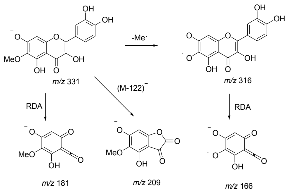
Figure 8. MS 2 fragmentation of patuletin 27 .
