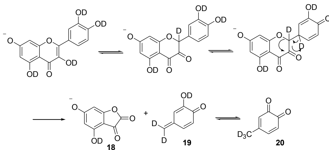
Figure 4. The (M-122)^{-} mechanism for 3',4'-dihydroxyflavonols.
