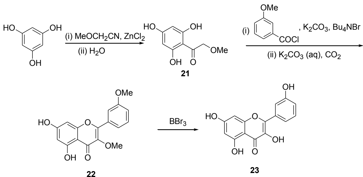
Figure 5. Synthesis of 23 .
