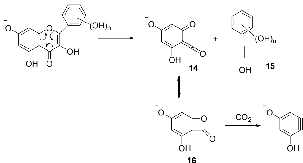
Figure 3. The RDA fragmentation mechanism.
