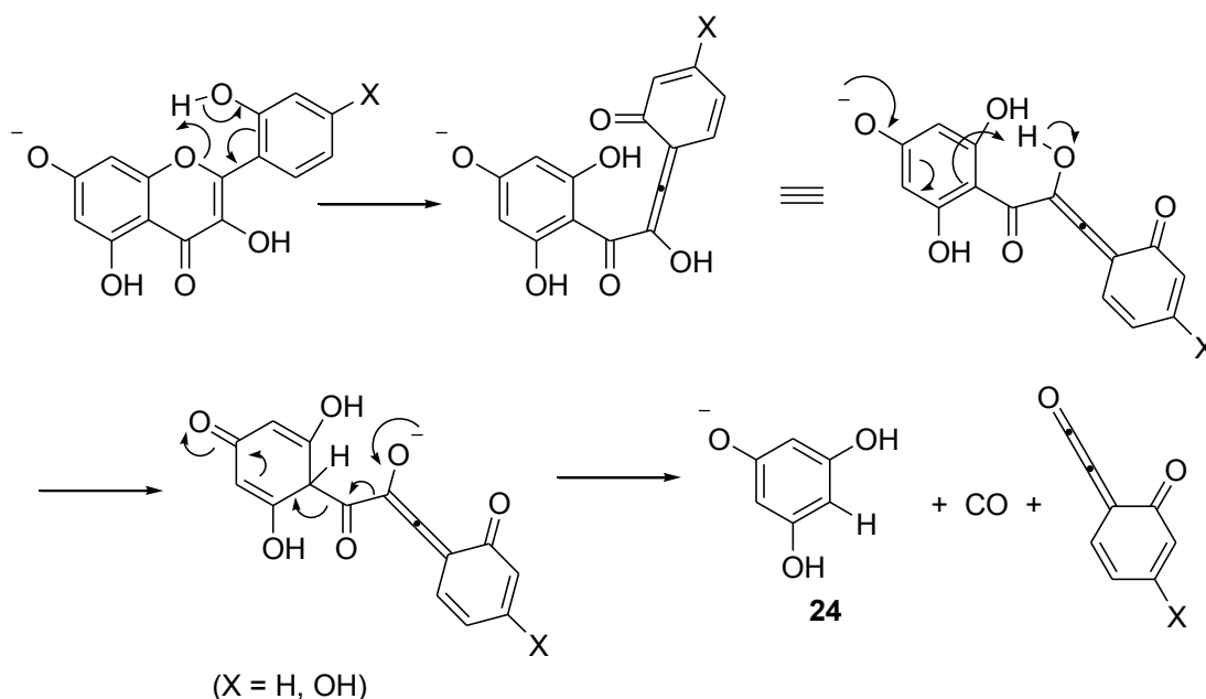
Figure 6. Formation of m/z 125 fragment ion in the negative ion ESI mass spectra of 2'-hydroxyflavonols.
