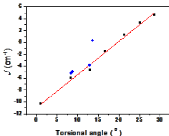
Figure 4. Magneto-structural correlation developed by varying the Mn-N-O-Mn angle in 1 ; blue stars represent the experimental J values for 1-4 .
