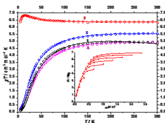
Figure 2. Plot of \chi_M T vs. T for complexes 1-4 . Inset: VTVH magnetisation data of 2 . Best-fit curves are shown as solid lines. See text for details.
