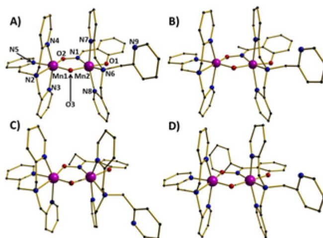
Figure 1. The molecular structures of 1-4 , A – D, respectively. Colour code: Mn = purple, O = red, N = blue, C = black. H-atoms, counter ions and solvent molecules are omitted for clarity.
