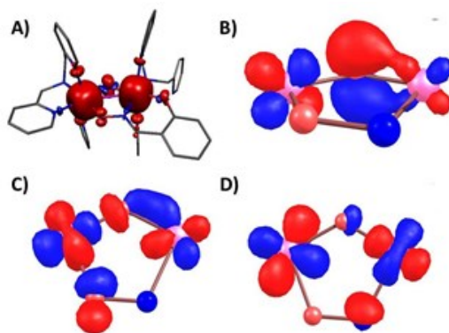
Figure 3. (a) Computed spin density plot for complex 1 . Qualitative MO diagram computed for complex 2 : (b) d_{xz} orbital; (c) d_{x^2-y^2} orbital (alpha); (d) d_{x^2-y^2} orbital (beta). For (b)-(d) the ligands and other atom contributions are removed for clarity. See Figure S2 for the complete picture.
