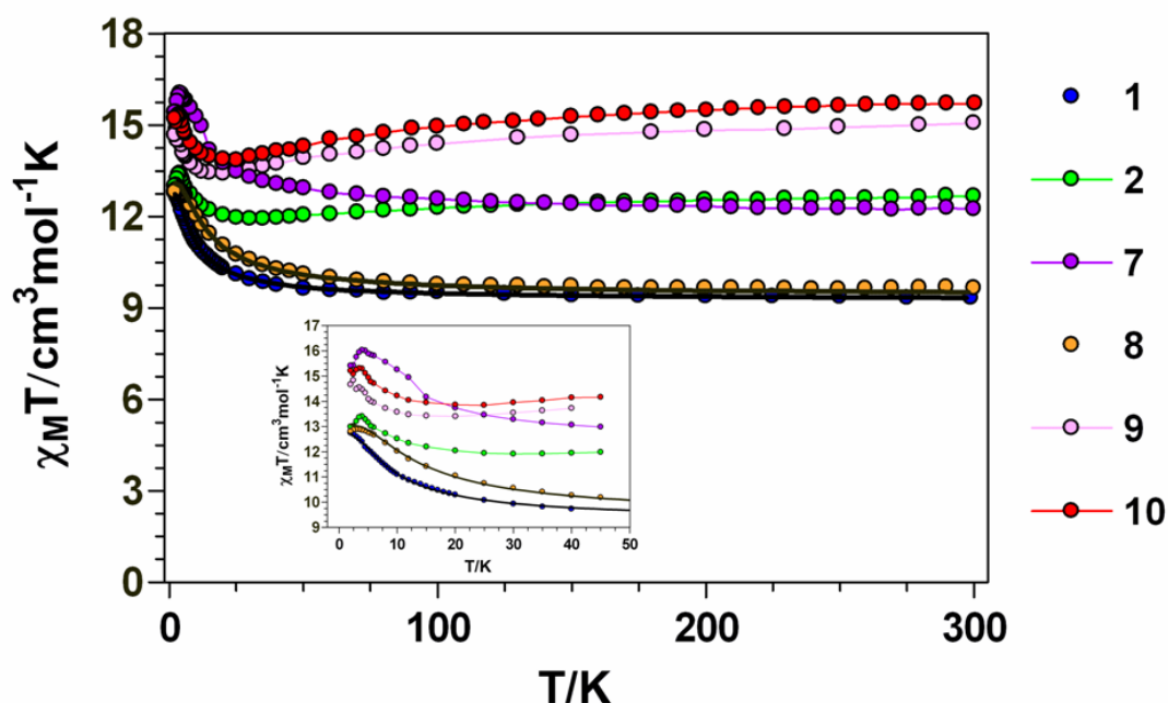
Figure 8. Temperature dependence of the \chi_{\text{M}}T product at 1000 Oe for complexes 1-2 and 7-10 . Inset highlights the low temperature data. Black solid lines show the best fits for complexes 1 and 8 . The rest of the solid lines are a guide to the eye.
