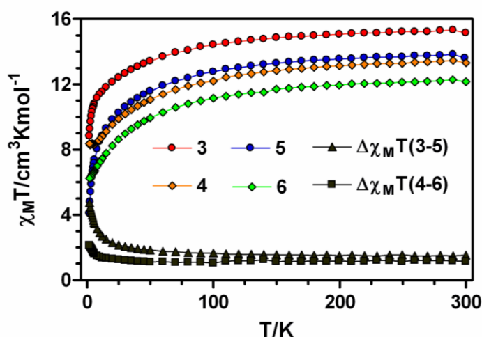
Figure 12. Temperature dependence of the \chi_{\text{M}}T product for 3-6 and the differences \Delta\chi_{\text{M}}T = (\chi_{\text{M}}T)_{\text{NiTb}} - (\chi_{\text{M}}T)_{\text{ZnLn}}
