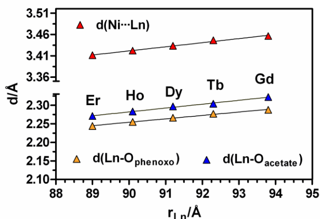
Figure 2. Plots of the Ni \cdots Ln , Ln \cdots O_{phenoxo} and Ln-O_{acetate} versus the Ln^{III} ionic radius.
