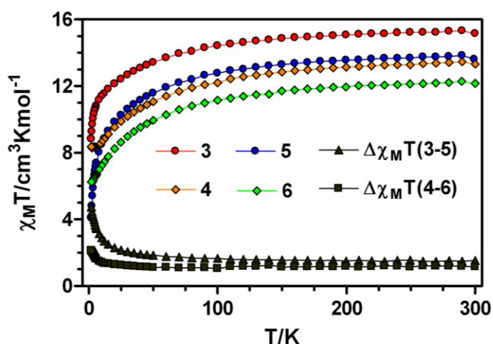
Figure 12. Temperature dependence of the \chi_M T product for 3-6 and the differences \Delta\chi_M T = (\chi_M T)_{\text{NiTb}} - (\chi_M T)_{\text{ZnTb}}
