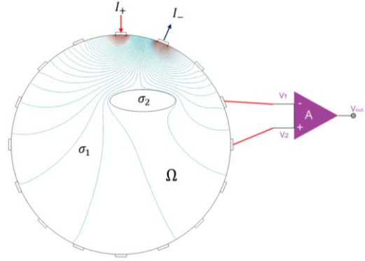
Fig. 2. Sensing principle of EIT.
