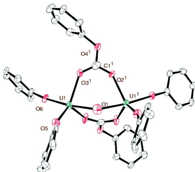
Figure 9. Thermal ellipsoid of (OTtbp) 2 U(μ-O)(μ-O 2 COTtbp) 2 U(OTtbp) 2 , 9 grown from benzene solution; probability 50 %, lattice solvent and tert -butyl groups omitted for clarity. Symmetry operator used to generate symmetry-generated atoms: y, x, -z .
