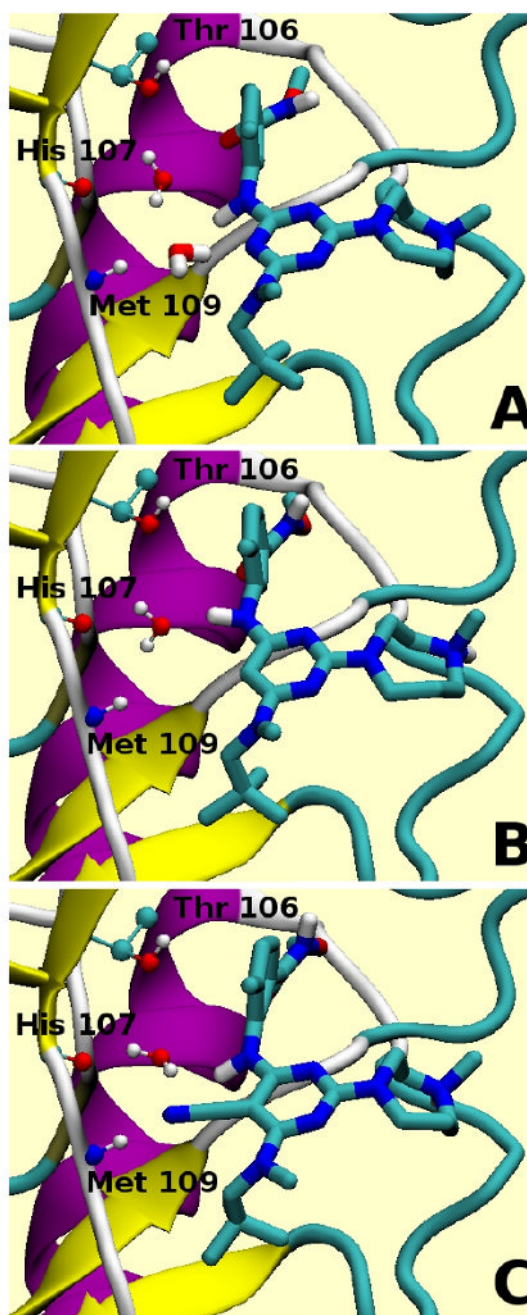
Figure 5. Location of key water molecules in the binding site of p38α MAP kinase in complex with, (A) 4 , (B) 6 , (C) 5 . The displaced water molecule is represented in sticks. For clarity, non-polar hydrogens and parts of the binding site have been omitted.
