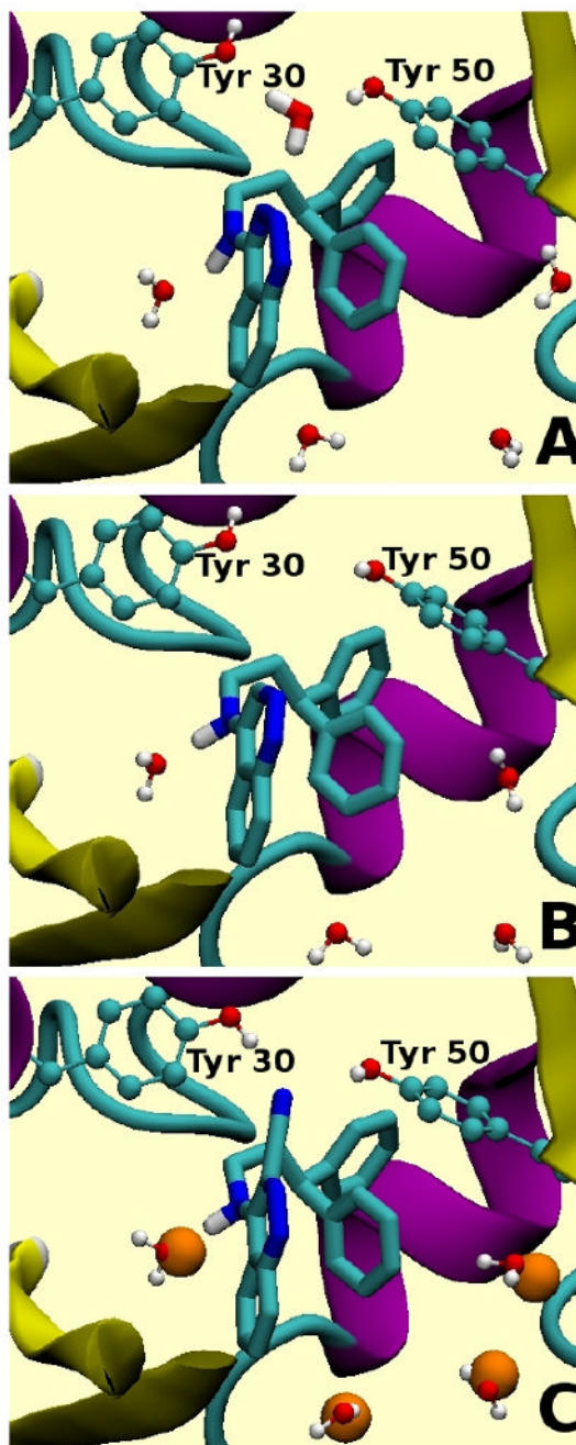
Figure 2. Location of selected water molecules in the binding site of scytalone dehydratase in complex with, (A) ligand 1 , (B) ligand 3 , (C) ligand 2 . The orange spheres indicate the position of water molecules observed in the crystal structure of 2 complexed to scytalone dehydratase. 37 The displaced water molecule is represented in sticks. For clarity, non polar hydrogens and parts of the binding site have been omitted. Figures created with VMD. 59
