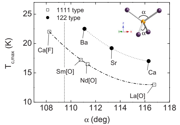
FIG. 9. (Color online) Variation in the superconducting T_c with tetrahedral As-Fe-As angle (defined in the inset) for well-characterized 122-type AE(\text{Fe}_{1-x}\text{Co}_x)_2\text{As}_2 (solid circles) and 1111-type R\text{Fe}_{1-x}\text{Co}_x\text{AsO} and A\text{EFe}_{1-x}\text{Co}_x\text{AsF} (open squares) superconductors. The line is intended as a guide for the eyes. Data were taken from the following references: Ca[F] (Ref. 18), La[O] (Refs. 13 and 17), Sm[O] (Ref. 17), Ca (Ref. 15), Sr (Ref. 16), and Ba (Ref. 39).
