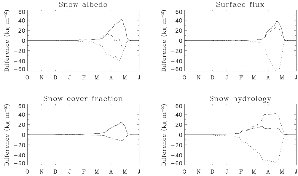
Figure 15: Differences between 2005-2006 ensemble mean snow mass and group means for configurations using snow albedo, surface flux, snow cover fraction and snow hydrology parametrization options 0 (solid lines), 1 (dashed lines) and 2 (dotted lines).
