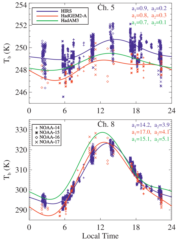
FIG. 1. Brightness temperatures in HIRS chs. 5 and 8 measured by HIRS and simulated from HadGEM2-A in July of 2002 to 2007 for the HadGEM2-A grid box centered on 31.25^\circ\text{N} , 1.25^\circ\text{E} . For HIRS each symbol represents a single measurement made within the grid box; for HadGEM2-A the symbols indicate the grid box value for the (hourly) output closest to the HIRS overpass time. The lines are the Eq. (1) Fourier fits to the data. The simulated fit for the 4\times larger HadAM3 grid box centered on 30.0^\circ\text{N} , 0.0^\circ is shown without symbols. The numbers are the fit parameters a_1 and a_2 . Lines and symbols are labeled on the top and bottom panels respectively. Note the different scales of the two y axes.
