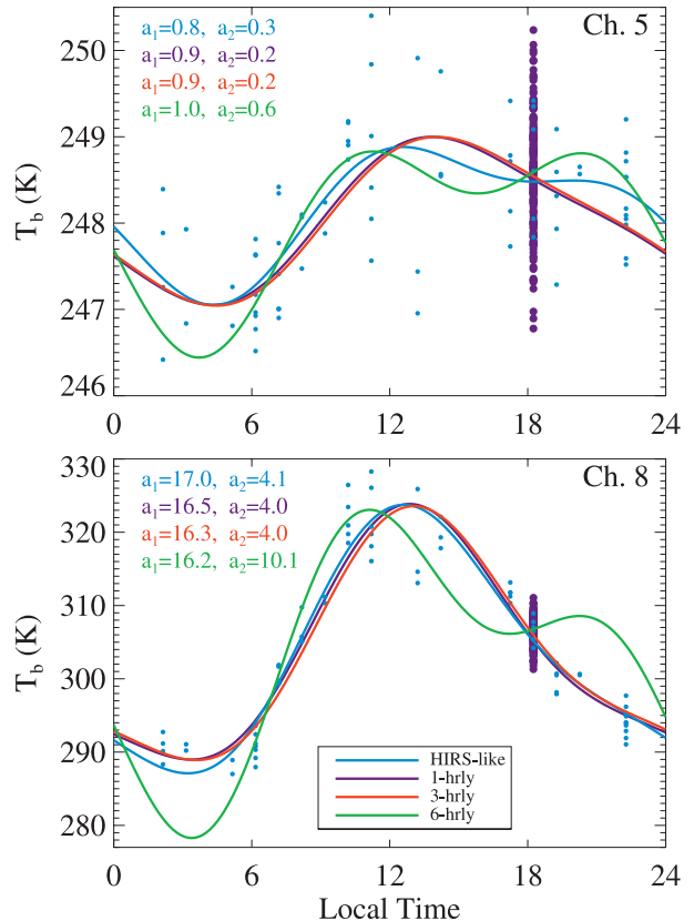
FIG. 9. Fourier fits to clear-sky brightness temperatures simulated from HadGEM2-A for the same channels, grid box, month, and integration period as Fig. 1. Fits are shown for 1-, 3-, and 6-hourly sampling of the model grid box along with the grid box sampled as seen by HIRS. Individual points are shown for the HIRS-like sampling and for the full model sampling at \sim 1800 local time. Individual points from other hours of the full sampling are omitted for clarity.
